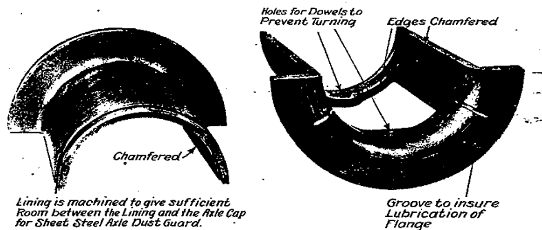
AXLE SUSPENSION BEARINGS
